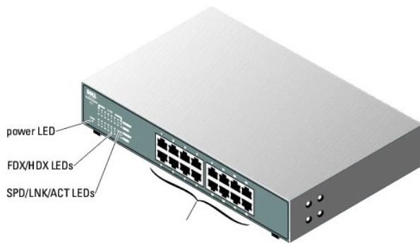
Figure 1-2. PowerConnect 2224
