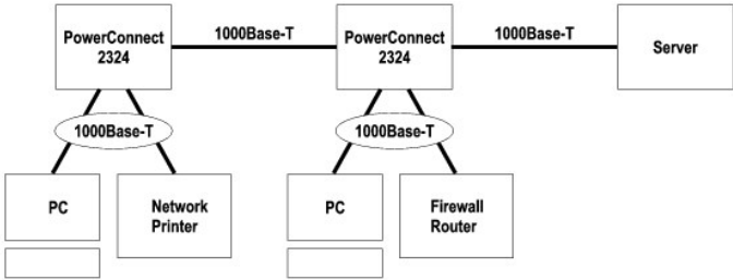
Figure 1-6. Large Workgroup
