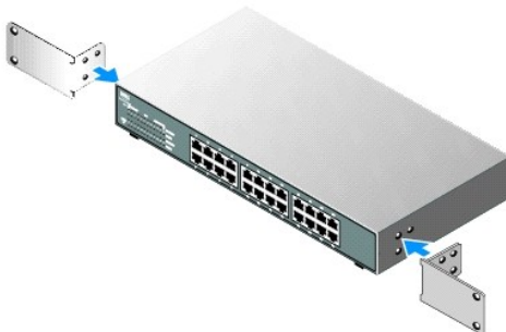
Figure 1-7. Brackets for Rack Installation
