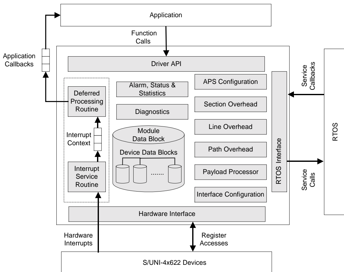
Figure 2: Driver Architecture
