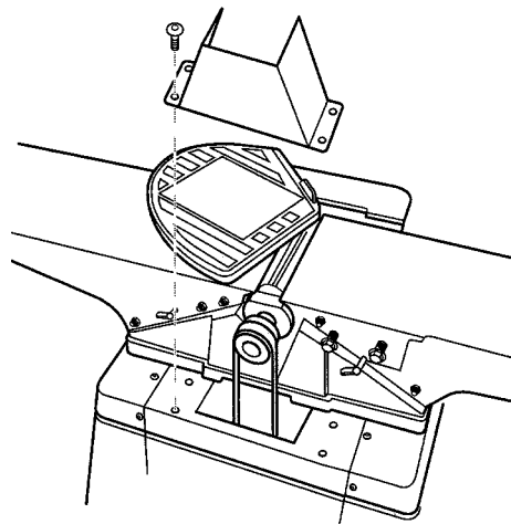
Belt Guard
