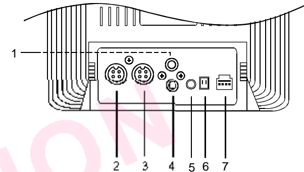
Fig. 3 Port connection
