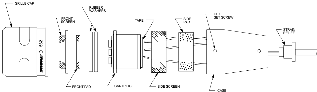
FIGURE 1 EXPLODED VIEW
