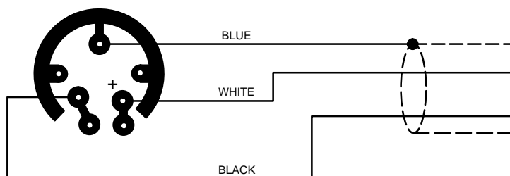
FIGURE 2 INTERNAL CONNECTIONS
