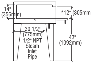
ER-12-5736 SIDE VIEW
