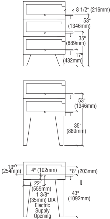
EP-EB-8-5736 SIDE VIEW
