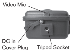
Fig. 1: Connections
