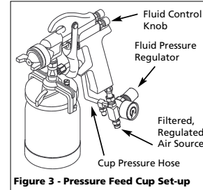
Figure 3 - Pressure Feed Cup Set-up
