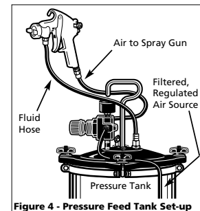
Figure 4 - Pressure Feed Tank Set-up
