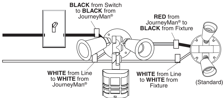
Wiring to a Motion Light & Standard Fixture
