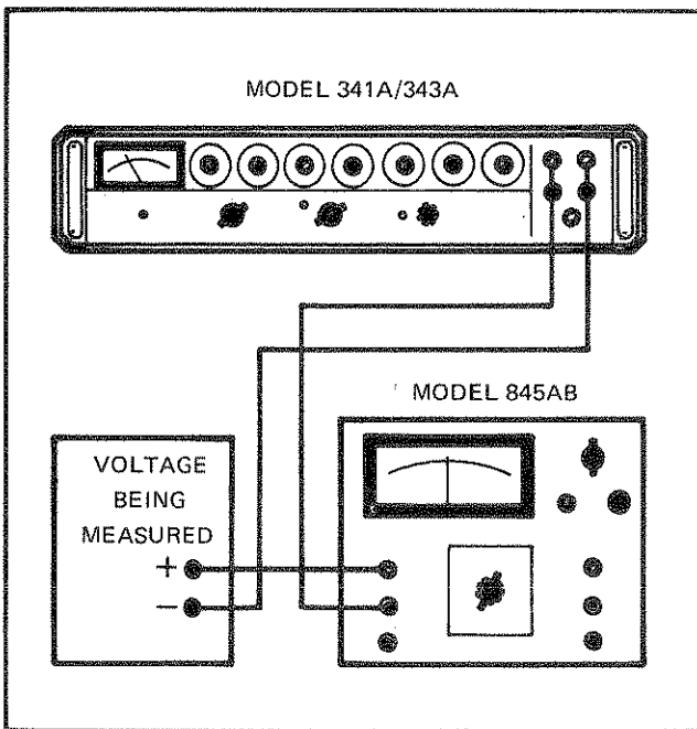
Figure 2-3. DIFFERENTIAL VOLTMETER
