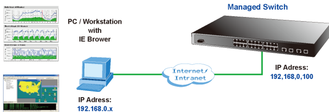
Figure 3-3: SNMP management
