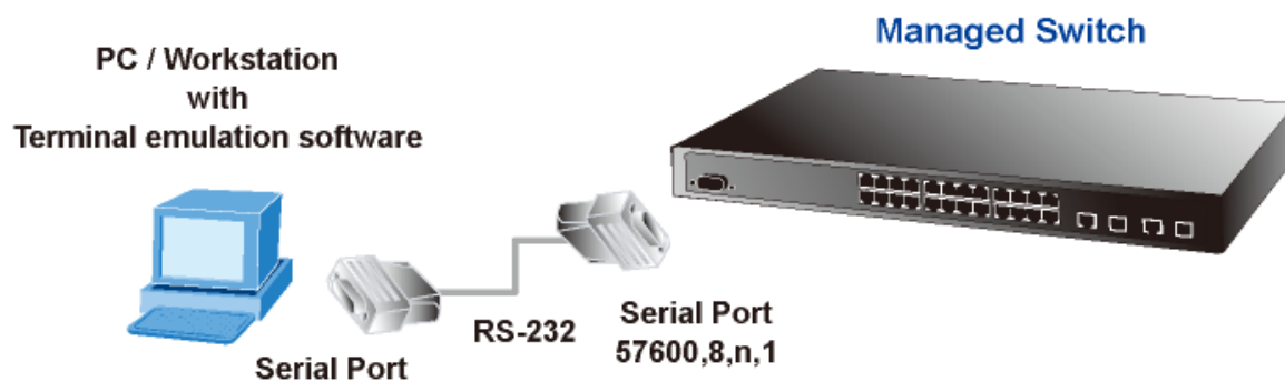
Figure 3-4: Console management setup
